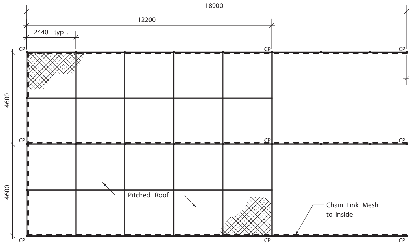
PLAN VIEW
