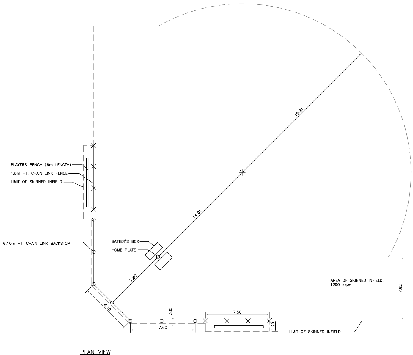
PLAN VIEW
