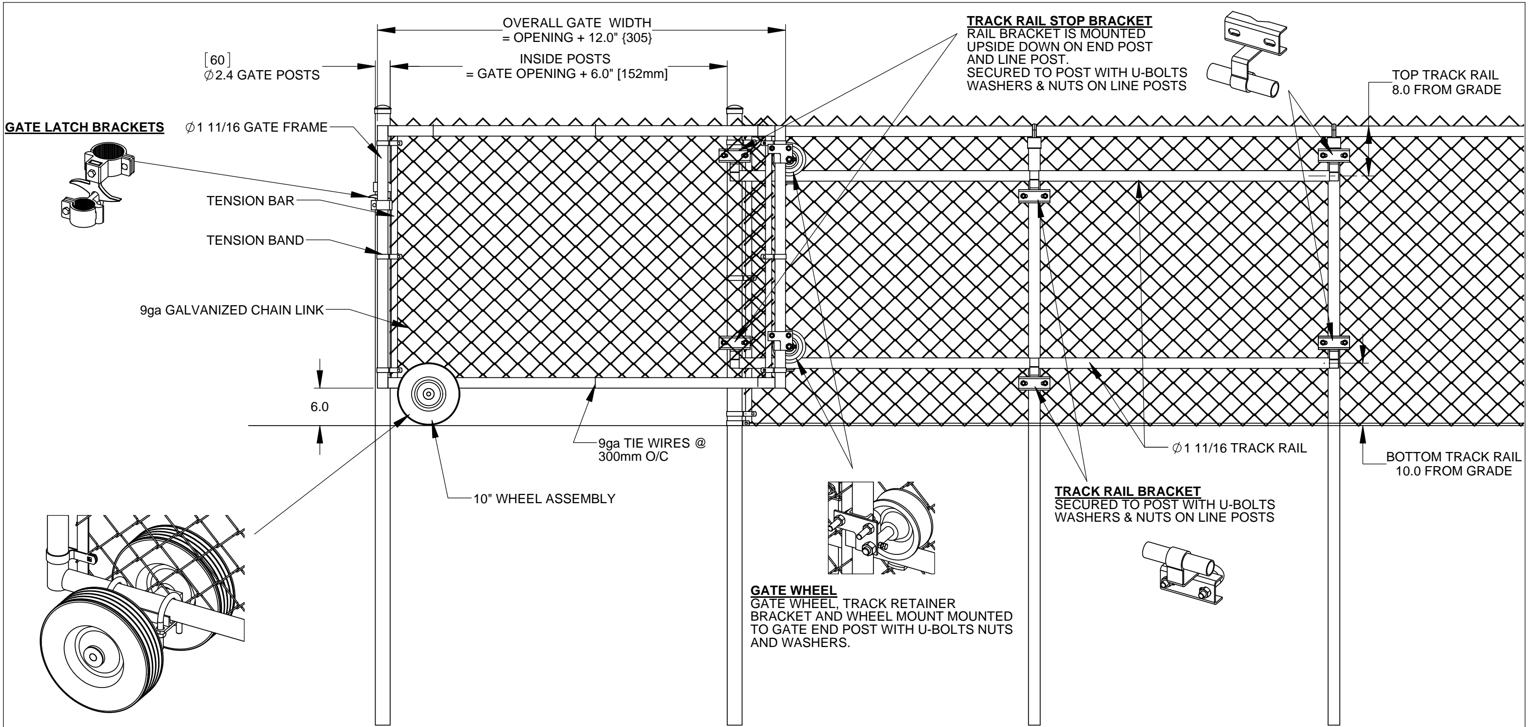
10" WHEEL ASSEMBLY SECURED TO GATE BOTTOM RAIL WITH U-BOLTS WASHERS & NUTS.
